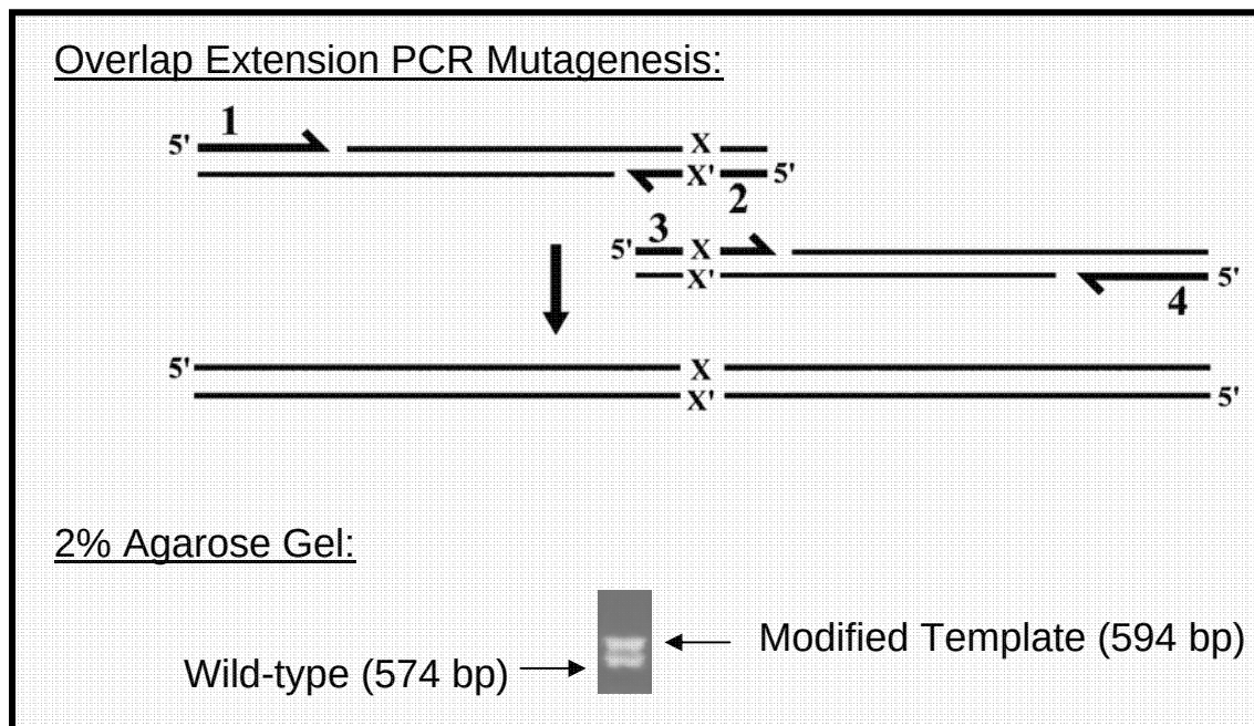
Figure 1. Panel A illustrates the construction of modified control template using
