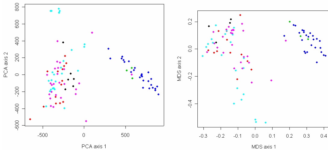
Figure 4.3 PCA and MDS plots of a small library of isolates where different colors indicate different source categories.
