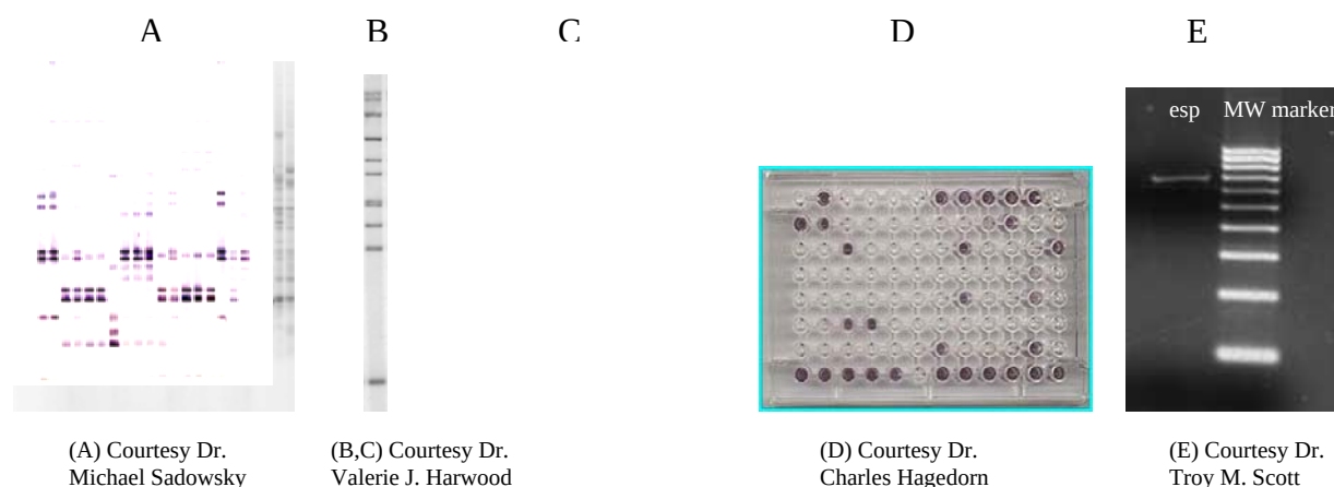
Figure 6.1 Illustration of some strains/patterns/markers (SPMs) currently utilized in MST methods. (A) rep-PCR patterns of E. coli isolates – each vertical lane represents one pattern. (B) ribotype pattern of one E. coli isolate (C) ribotype patterns of Enterococcus isolates (D) carbon source utilization pattern of one Enterococcus isolate (E) specific genetic marker ( esp of E. faecium ) amplified by PCR of Enterococcus DNA
